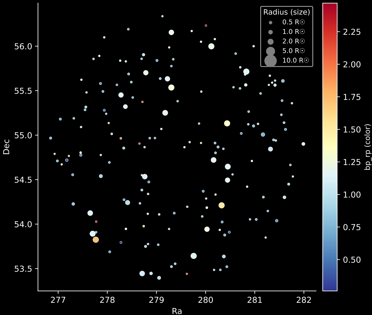
APOGEE DR17 Field: [139+61_MGA] Stars: 169
