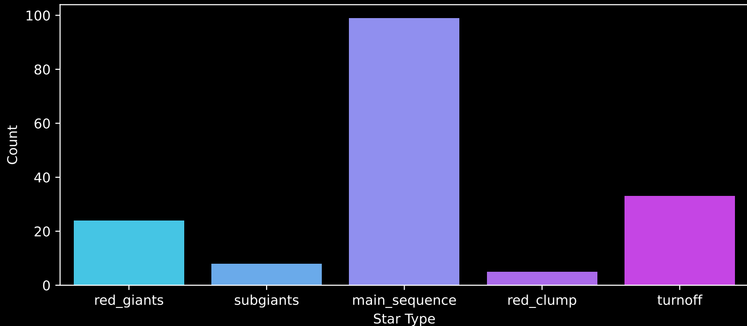
APOGEE DR17 Field: [139+61_MGA] Count plot of Star Type
