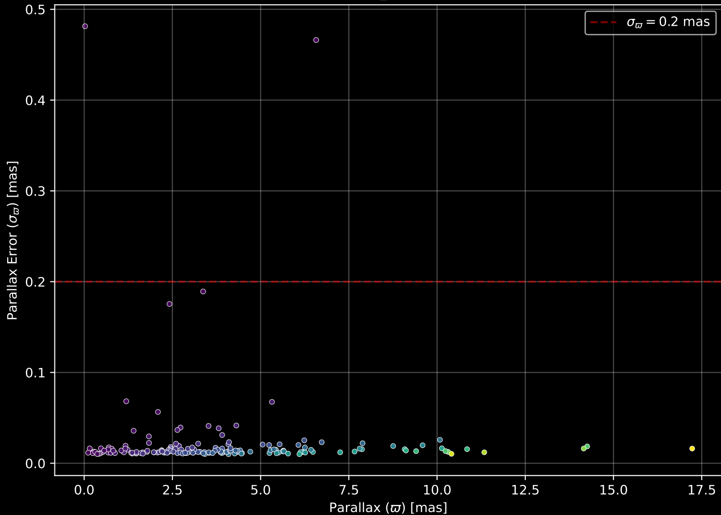
APOGEE DR17 Field: [139+61_MGA] Parallax Quality (n= 169)
