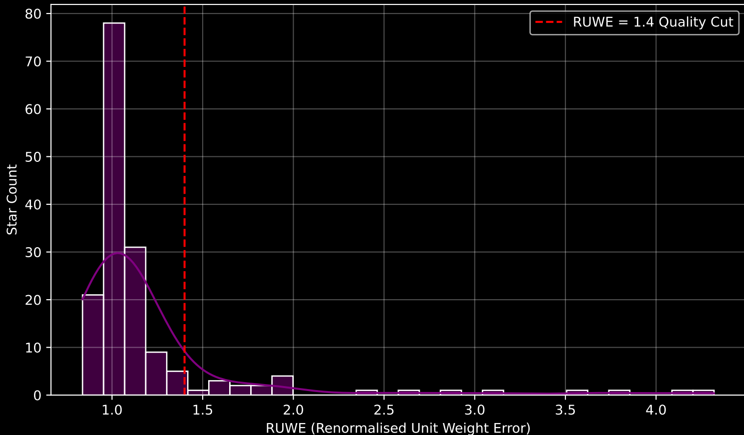
GAPOGEE DR17 Field [139+61_MGA] RUWE Distribution (n= 164)
