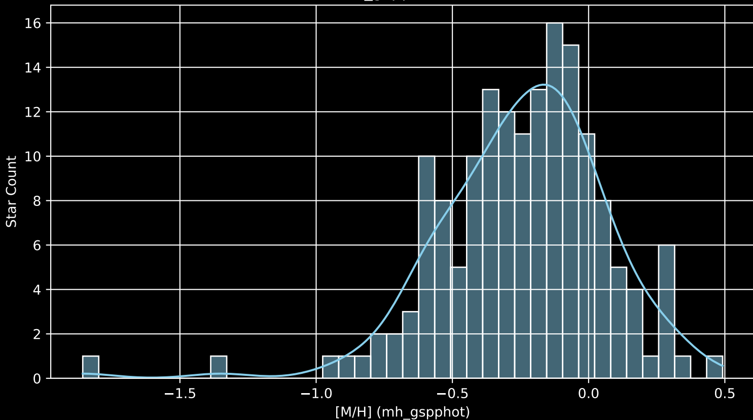
APOGEE DR17 Field: [139+61_MGA [M/H] (mh_gspphot) (n= 162)
