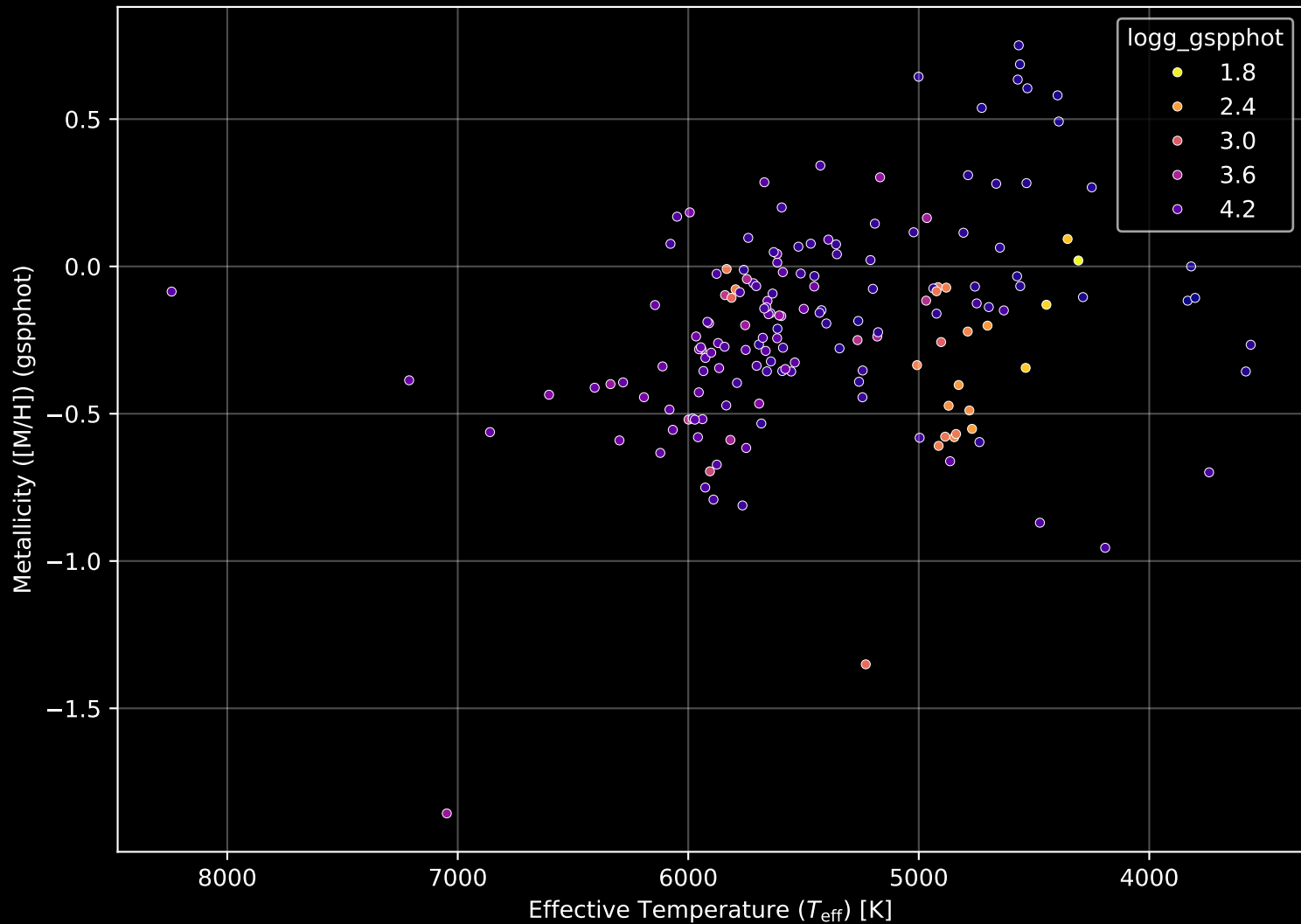
APOGEE DR17 Field: [139+61_MGA] Stellar Population Parameters (n= 169)
