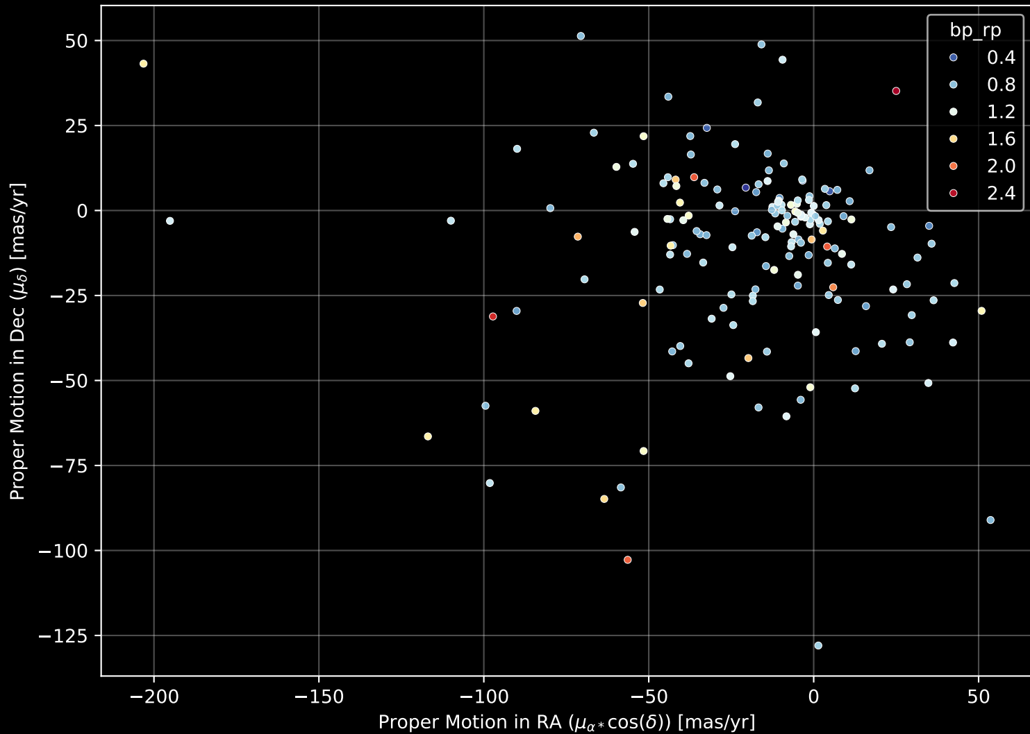
APOGEE DR17 Field: [139+61_MGA] Proper Motion Diagram (n= 169)
